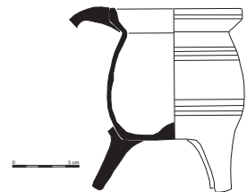
Pot tripode 4147.03 (A. Vignet)
